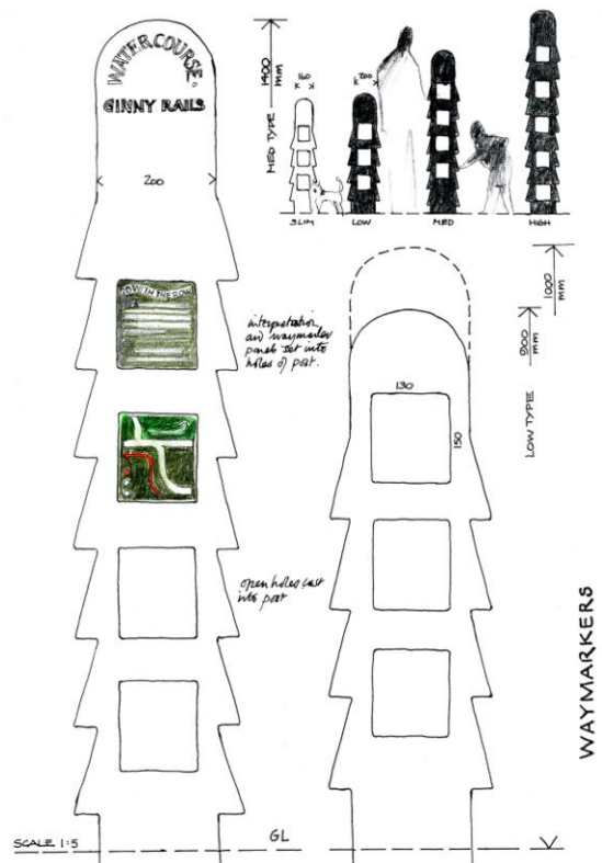
The concept designs for the way-markers and posts were developed from old sluice gearing that we discovered on site.
